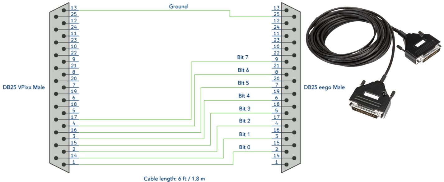
Simplified Schematic VPiXX DB25 Digital Out to ANT Neuro eego Amplifier DB25 Digital Input
