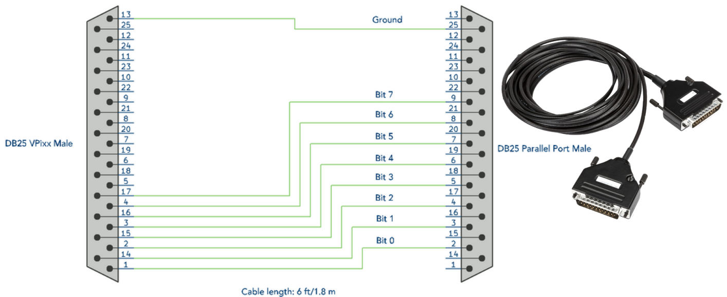
Simplified Schematic VPiXX DB25 Digital Out to DB25 Parallel Port
